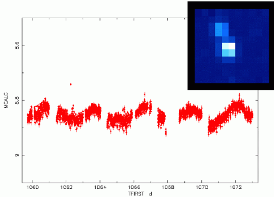
Figure 14: OMC light curve of the high-mass X-ray binary Cygnus X-1 obtained using single exposures of 10 and 30 s. The OMC sub-window for this source is shown on the upper right corner of the graph. Time is in INTEGRAL Julian days. (Credits: OMC Team).
