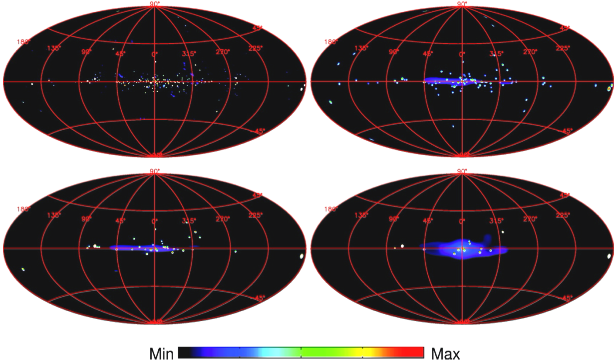
Figure 14 – SPI sky maps in the 25-50 keV (top, left), 50-100 keV (top, right), 100-200 keV (bottom, left) and 200-600 keV (bottom, right) energy bands. The images are scaled logarithmically with a rainbow colormap. The scale is saturated to reveal the weakest sources. At low energy, the sky emission is dominated by sources, while a "diffuse/extended" structure appears above 200-300 keV, in a domain corresponding to the annihilation radiation. These images have been obtained by maximum-likelihood fitting of point sources from a reference catalogue, plus diffuse-emission models represented from a set of pixons (16×2.6 deg in size). From Bouchet et al. 2008, ApJ 679, 1315.
