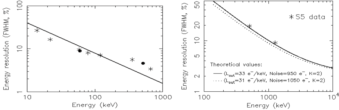
Figure 11. Left panel: The energy resolution of ISGRI. The solid line shows the theoretically expected values, and the stars are values measured before launch using an engineering model. The study of the in-flight W fluorescence line at 60 keV and the e^+e^- annihilation lines at 511 keV (shown as filled circles) do not reveal any evidence of a change of the ISGRI spectral performance. Right panel: The energy resolution of PICsIT at 511 and 1275 keV as measured in-flight using Calibration Unit (S5) data (shown as stars). Also shown are the theoretical expectations as determined from pre-flight tests using an engineering model. The electronic-noise values (“Noise”) refer to one ASIC only; a 10% increase is expected when extrapolating to the complete detector electronic chain.
