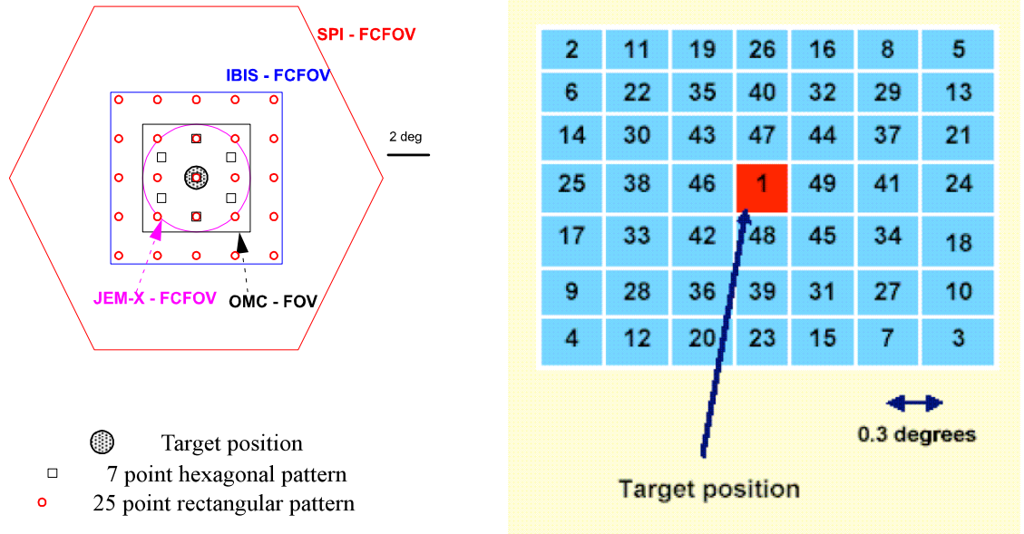
Figure 3: Schematic view of dithering patterns (left) and COP Offset Pattern for a 5x5 dither.
