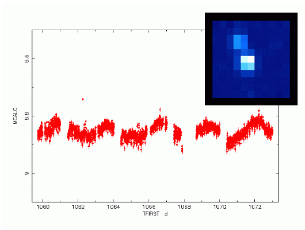
Figure 13: OMC light curve of high-mass X-ray binary Cyg X-1 obtained using single exposures of 10 and 30 seconds. The OMC sub-window for this source is shown on the upper right corner of the graph. Time is in INTEGRAL Julian days. (Credits: OMC Team)
