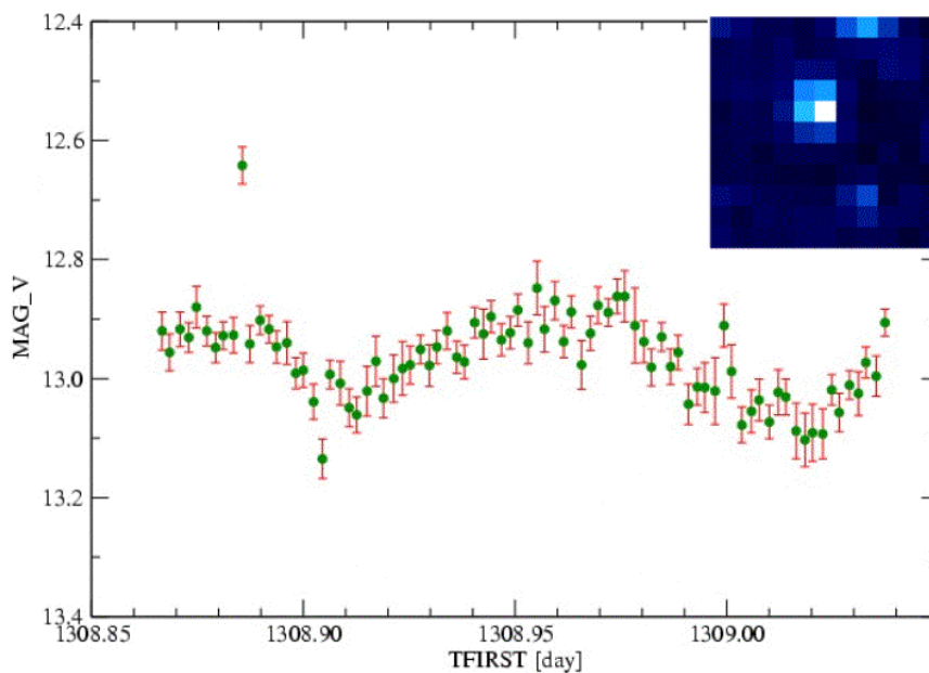
Figure 14: OMC light curve of the low-mass X-ray binary Sco X-1. It is based on single exposures of 100 seconds. The OMC sub-window for this source is shown on the upper right corner of the graph. Time is in INTEGRAL Julian days. (Credits: OMC Team)
