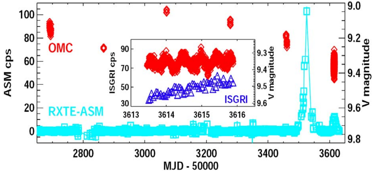
Figure 17: Long-term light curves of the Be/X-ray binary and accreting pulsar 3A0535+262/HD 245770 obtained with the RXTE/ASM (left Y-axis) and the INTEGRAL/OMC (right Y-axis). The inset shows the OMC and ISGRI light curves during the INTEGRAL Target of Opportunity observations around MJD 53613-53616. (Taken from Kretschmar et al. 2006, ESA SP-604, p. 273)
