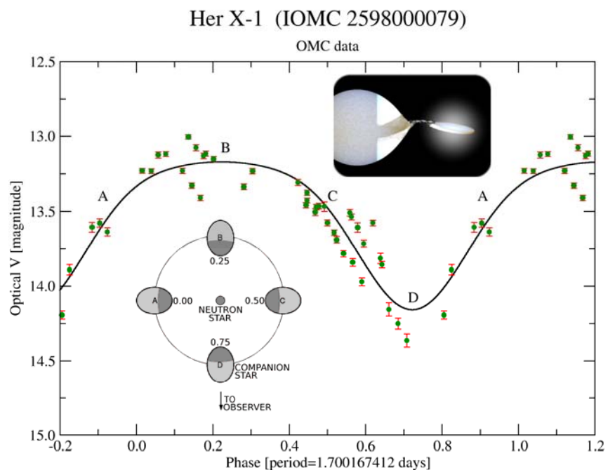
Figure 16: OMC light curve of the low-mass X-ray binary Her X-1 (see Figure 15) folded on the 1.7 days orbital period (Risque et al. 2008, PoS(Integral08)129).
