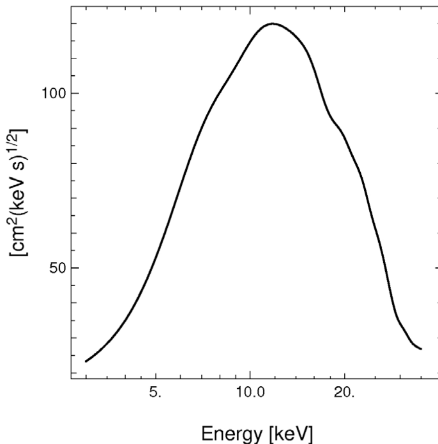
Figure 18: C-factor for estimating the continuum sensitivity for the combined JEM-X units for an on-axis source (see formula in Section 5.4).
