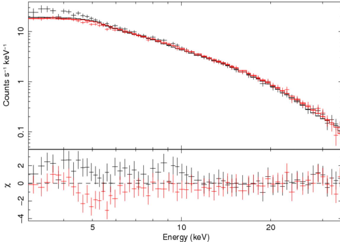
Figure 14: JEM-X1 (black) and JEM-X2 (red) Crab count spectra together with the simultaneous fit to a power-law emission model, dN/dE=N(E/1 \text{ keV})^{-\Gamma} \text{ ph cm}^{-2} \text{ s}^{-1} \text{ keV}^{-1} , subjected to photo-electric absorption of 0.36 \times 10^{22} \text{ atoms cm}^{-2} , with N is 6.65 \text{ ph cm}^{-2} \text{ s}^{-1} \text{ keV}^{-1} and \Gamma is 2.0. The data are from revolution 39 with a total exposure time of 1.2 ksec. A systematic error of 3% has been added. The goodness-of-fit is \chi^2=149 for 126 degrees of freedom.
