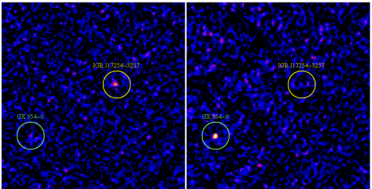
Figure 17: JEM-X 3-10 keV images obtained during a 45 s exposure around the X-ray burst from IGR J17254-3257 (left) and over the whole science window (right).
