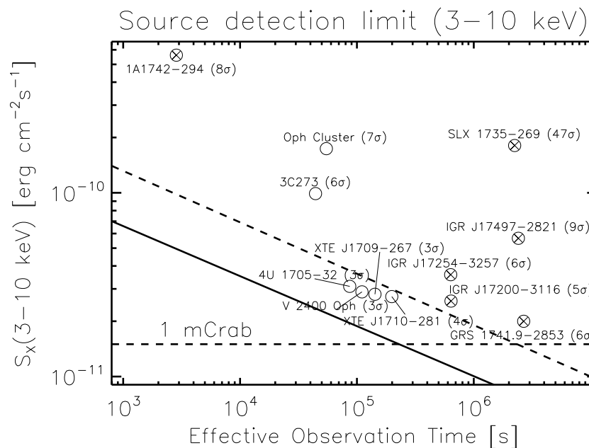
Figure 10: Source detection capabilities in the 3–10 keV energy band as a function of the effective accumulated exposure time in JEM-X mosaic images corrected for dead time, grey filter and vignetting effects. The slope of the lines is obtained from simulations where an isolated source must be detected at 6\sigma in the deconvolved image. The dashed line represents the case where there are additional sources in the field of view giving a background corresponding to a total of 1 Crab. The positions of the lines are determined by actual measurements. Examples of such actual observations are given: the source 3C 273 and the other empty circles are instances of isolated sources, while the crossed circles represent sources observed in the crowded Galactic Centre region. The \sigma values given in parentheses are obtained from a measure of the highest source pixel in significance mosaic maps with the default pixel size ( 1.5' ).
