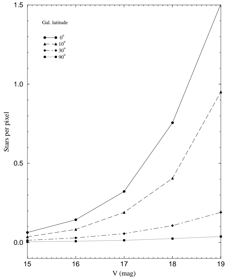
Figure 7: Average number of stars per pixel brighter than a given V magnitude at different galactic latitudes.
