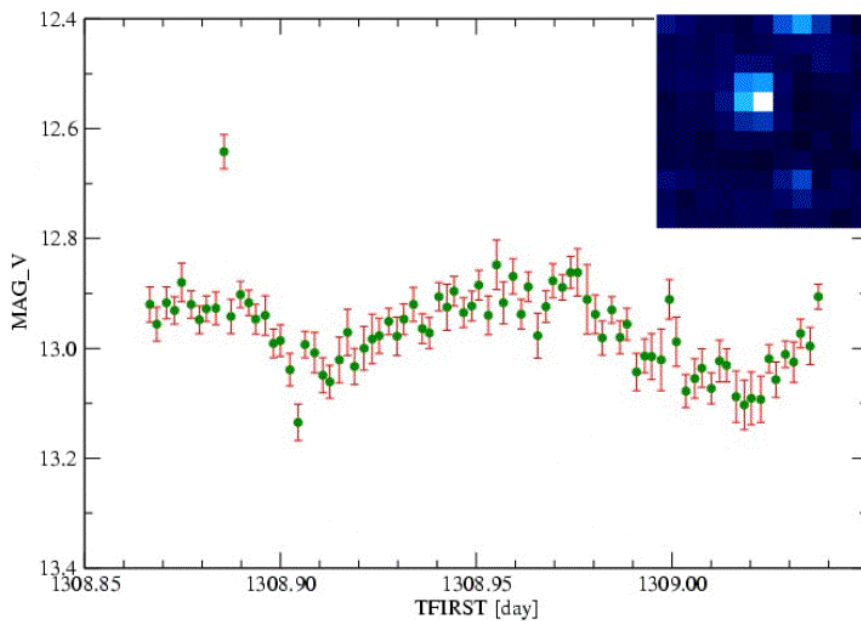
Figure 14: OMC light curve of the low-mass X-ray binary Sco X-1. It is based on single exposures of 100 seconds. The OMC sub-window for this source is shown on the upper right corner of the graph. (Credits: OMC Team)
