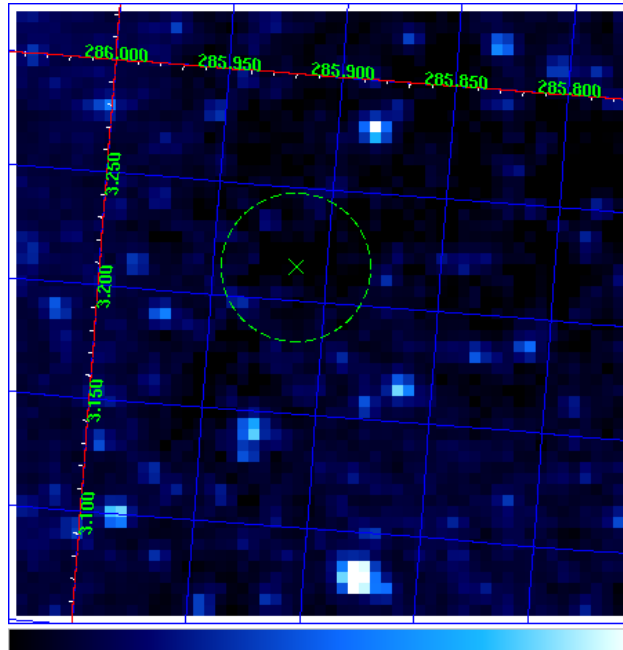
Figure 5: This image corresponds to the High Mass X-ray Binary 4U 1901+03, which generated a mosaic of 5x5 OMC sub-windows (16'x16'). The green cross and circle are the position and error of 4U 1901+03 in the IBIS
