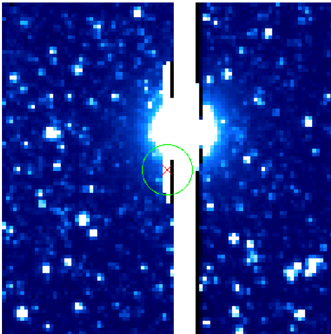
Figure 6: The only GRB observed by the OMC, on 2005 July 26. The red cross marks the position of the GRB, within the error circle in green. Unfortunately, the GRB happened to be close to a very bright, 0.8 magnitude in V, star (Alpha Crucis). The bright star completely saturated the CCD, causing the white vertical strip, and therefore completely contaminating the GRB emission.
