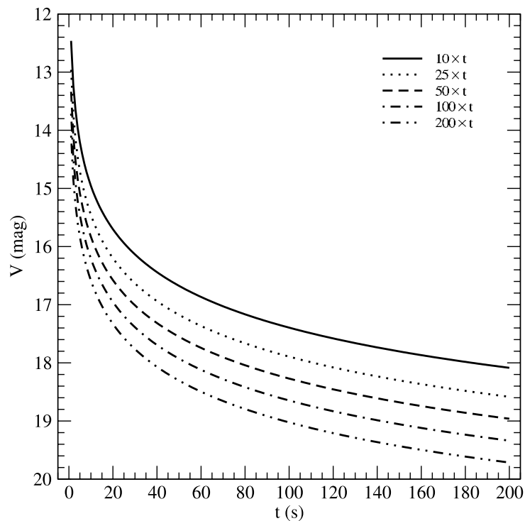
Figure 9: Limiting faint magnitude for a 3\sigma detection in the V band as a function of integration time. Best case background conditions are assumed (galactic pole, no zodiacal light). The curves correspond to different total numbers of images being combined.
