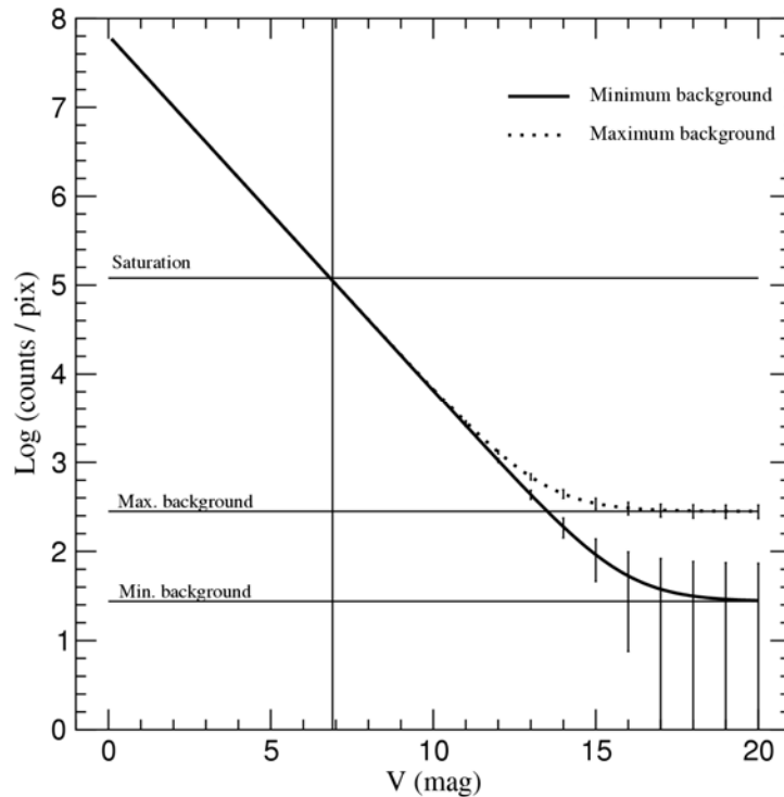
Figure 10: Expected number of counts on the central brightest pixel as a function of V magnitude, for an integration time of 10 sec. The error bars correspond to 1\sigma . The plot also includes the expected background flux computed for maximum and minimum conditions.
