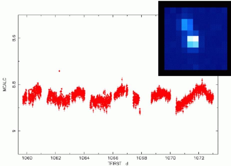
Figure 13: OMC light curve of high-mass X-ray binary Cyg X-1 obtained using single exposures of 10 and 30 seconds. The OMC sub-window for this source is shown on the upper right corner of the graph. (Credits: OMC Team)
