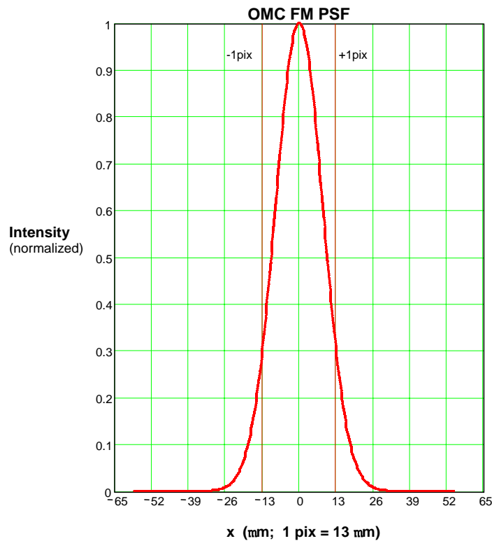
Figure 12: Point Spread Function of the OMC (optical system + detector). The plot shows a fit to the average PSF measured under different conditions. The PSF measured in orbit follows a Gaussian with FWHM \approx 1.3 pixels. More than 90% of the energy falls within 3 \times 3 pixels.
