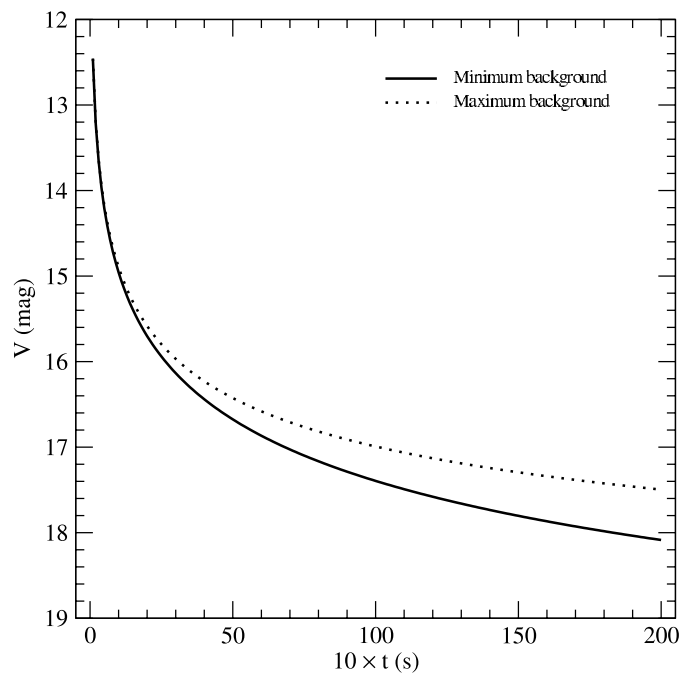
Figure 8: Limiting faint magnitude for a 3\sigma detection in the V band as a function of integration time. The best and the worst background cases are shown. It is assumed that 10 separate exposures, each with the integration time as given in the plot, have been combined together in order to increase the signal to noise ratio.
