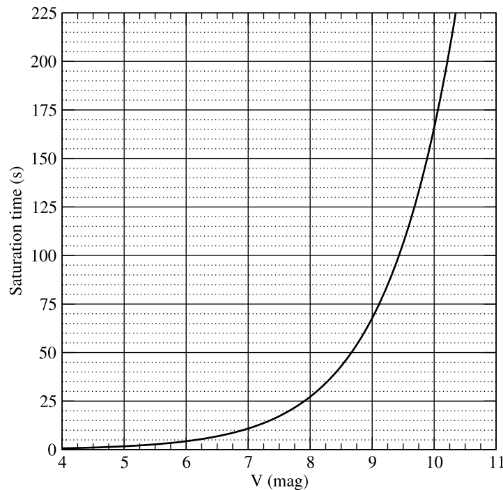
Figure 11: CCD saturation time as a function of V magnitude. Note that for integrations of 50 sec, all stars with m_V < 8.6 will saturate the CCD. For the shortest OMC integration times (fast monitoring mode: 3 sec), the brightest stars that can be observed should be fainter than m_V > 5 .
