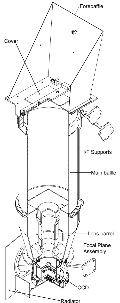
Figure 2: A 3-D cut of the OMC Camera Unit.
