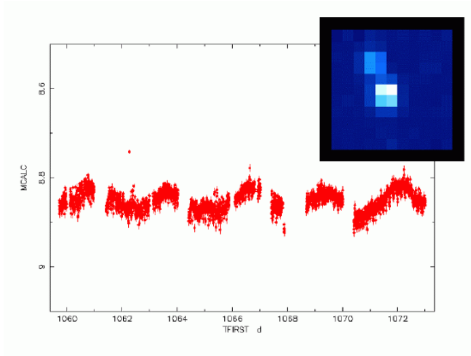
Figure 13: Computed light curve for Cyg X-1 using single exposures of 10 and 30 seconds. The OMC sub-window for Cyg X-1 is shown on the upper right corner of the graph.
