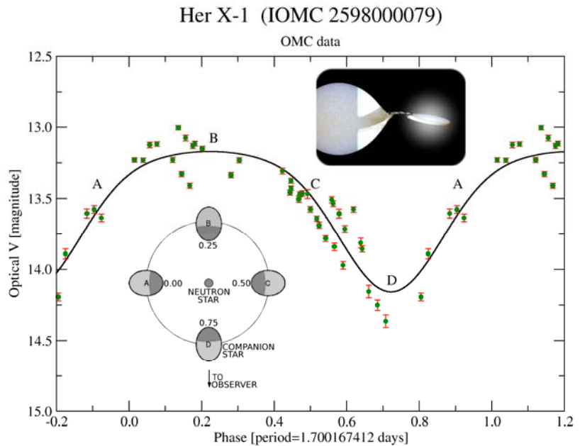
Figure 16: OMC data of Her X-1 (see Figure 15) folded on the 1.7 days orbital period. The optical variations are due to the tidal distortion of the companion star, and to the intense X-ray heating of the illuminated face of the companion produced by the neutron star. The insets show an artist's impression of the system and a sketch of the situation at different orbital phases (the orbit is almost circular) - not to scale and omitting the accretion disk:
