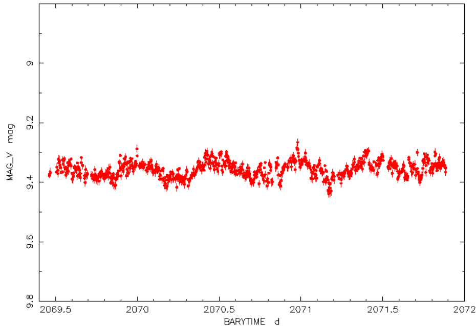
Figure 17: OMC light curve during an INTEGRAL TOO observation of the Be/X-ray binary 3A 0535+262, obtained by using single exposures of 10 and 50 seconds. It shows small variability typical of Be systems.
