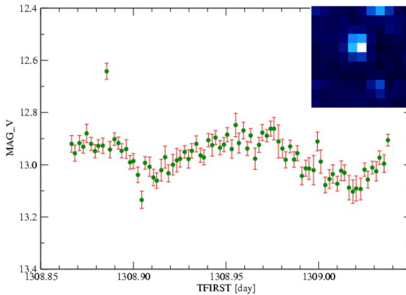
Figure 14: OMC light curve of the low-mass X-ray binary Sco X-1. It includes only single exposures of 100 seconds. The downloaded OMC sub-window for this source is also shown on the upper right corner of the graph.
