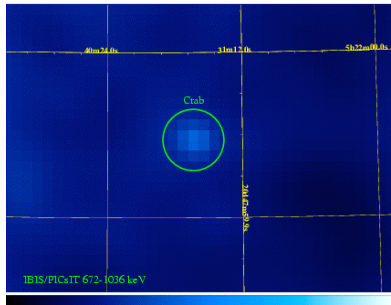
Figure 15. IBIS/PICsIT image of the Crab in the “MeV” range (672-1036 keV), using data based on 625 ks of net exposure time.
