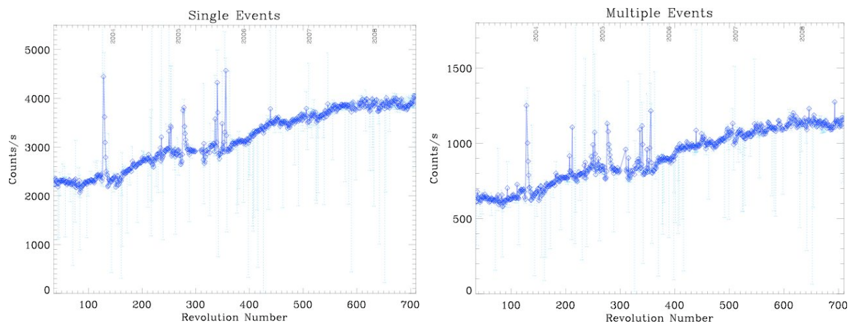
Figure 8. Total PICsIT count rate as a function of time (revolution number), computed with OSA 7 at the science window level. The left panel shows the count rate for all single events and the right panel shows the count rate for multiple events.
