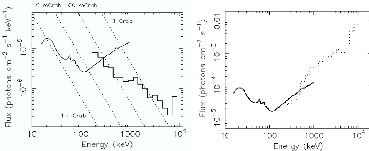
Figure 16. Overall IBIS 3σ continuum (left; 10 5 s) and narrow line (right; 10 5 s) sensitivity derived from empty field observations, and continuum binned to ΔE=E/2. Systematic errors (such as background uniformity) are not taken into account. ISGRI is from 15 to 1000 keV and PICsIT from 200 to 10 4 keV (single and multiple). Reference fluxes are for a power-law Γ=-2.
