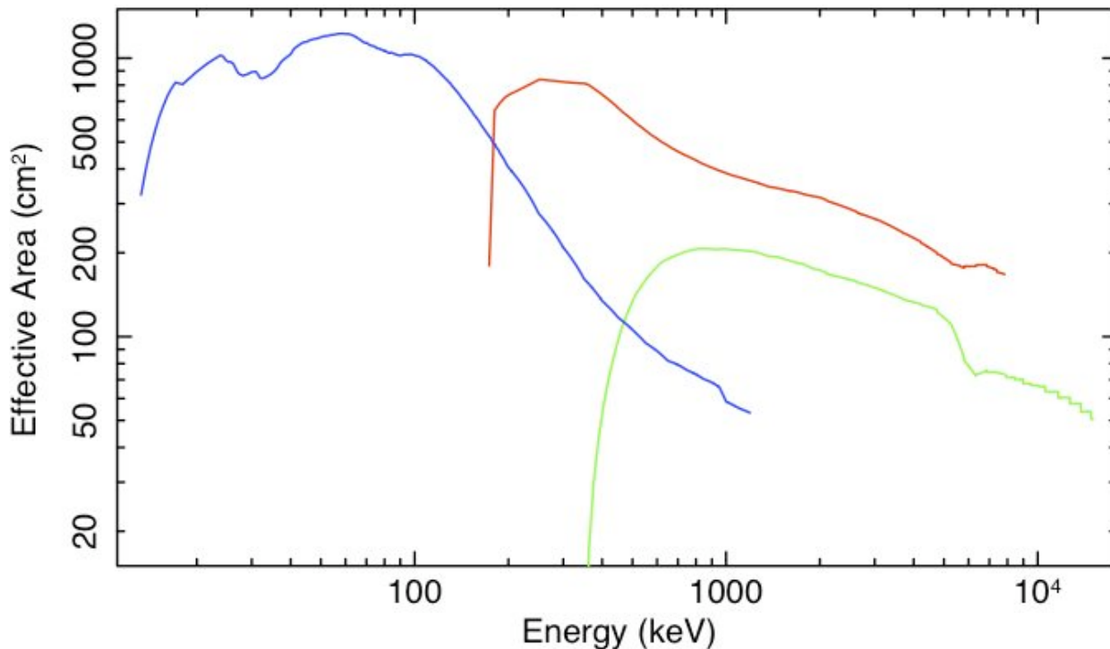
Figure 1: Effective area: ISGRI (blue) and PICsIT (single: red, multiple: green. See § 3.1).
