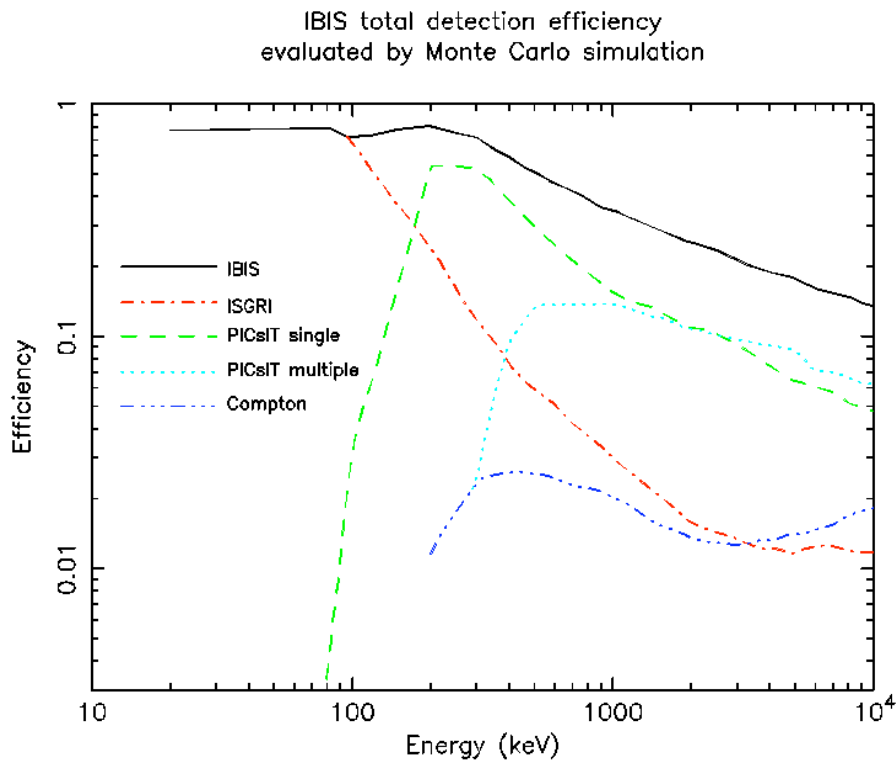
Figure 5. IBIS efficiency for the different detection techniques.
