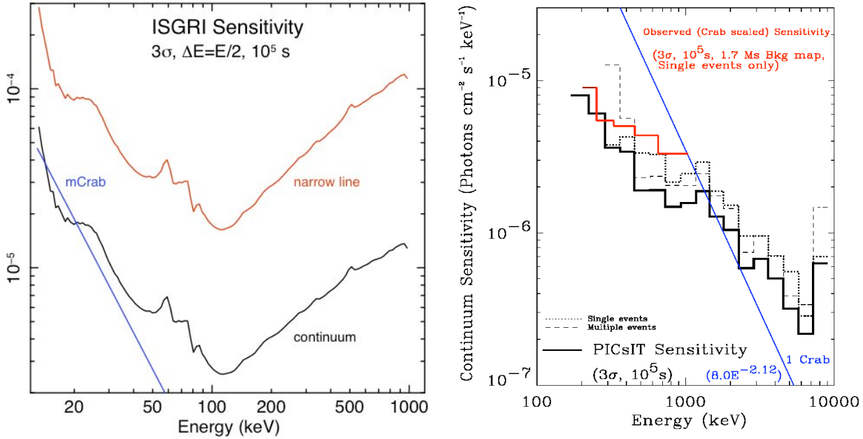
Figure 15. Left: Most recent update to ISGRI continuum (black: in Photons/cm 2 /s/keV) and narrow line (red: in Photons/cm 2 /s) sensitivity derived from 77 ks of empty field observations processed with OSA 7. Right: PICsIT statistically limited continuum sensitivity is given by the black histograms, from single events (dotted), multiple events (dashed), and combined (solid), all scaled to the in-flight background count rate, and compared with the sensitivity obtained by scaling from the Crab observation using OSA 5 (red; single events only). All sensitivities are for 10 5 s exposure time, 3σ detection and continuum binned to ΔE= E/2.
