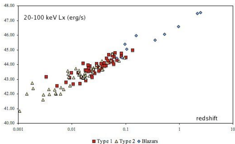
Figure 14. Luminosity (20-100 keV) versus redshift for AGN with known distance. The sample is taken from the third INTEGRAL/IBIS survey.
