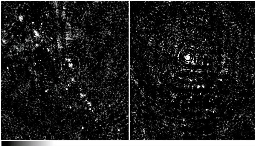
Figure 8. A comparison between two significance mosaics (18-25 keV) of equal exposure (~2 Ms) obtained from observations done with the 5x5 dithering mode (left, Galactic Center field) and the hexagonal dithering mode (right, GRS 1915+105 field). The significance scale runs from 2 to 50\sigma . OSA software version 5.1 has been used. Clearly, the mosaic derived from hexagonal dither mode observations still suffers from a systematic circular effect on a large spatial scale, despite improvements in the analysis procedures.
