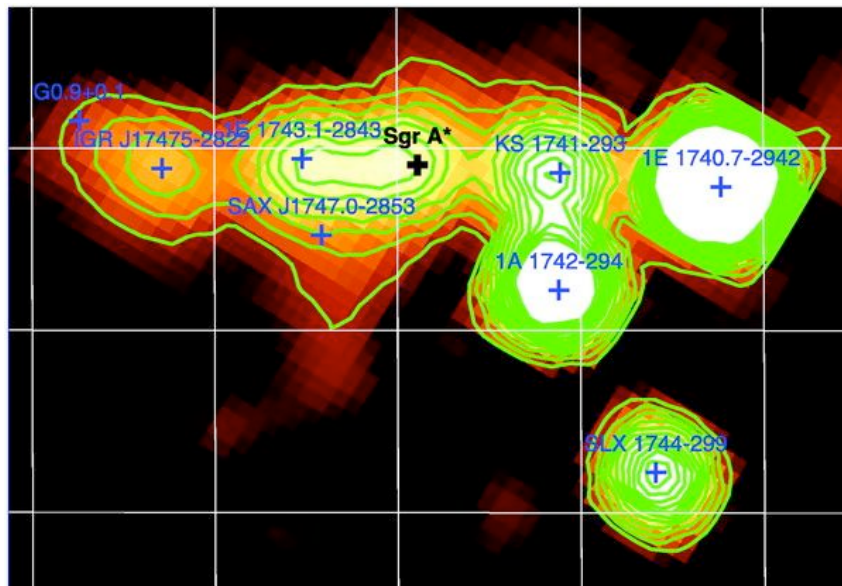
Figure 13. IBIS/ISGRJ significance mosaic in the 20-40 keV band, using 7 Ms of data, with an effective exposure of 4.7 Ms at the position of Sgr A*. The angular scale is about 2.5^\circ \times 1.5^\circ .
