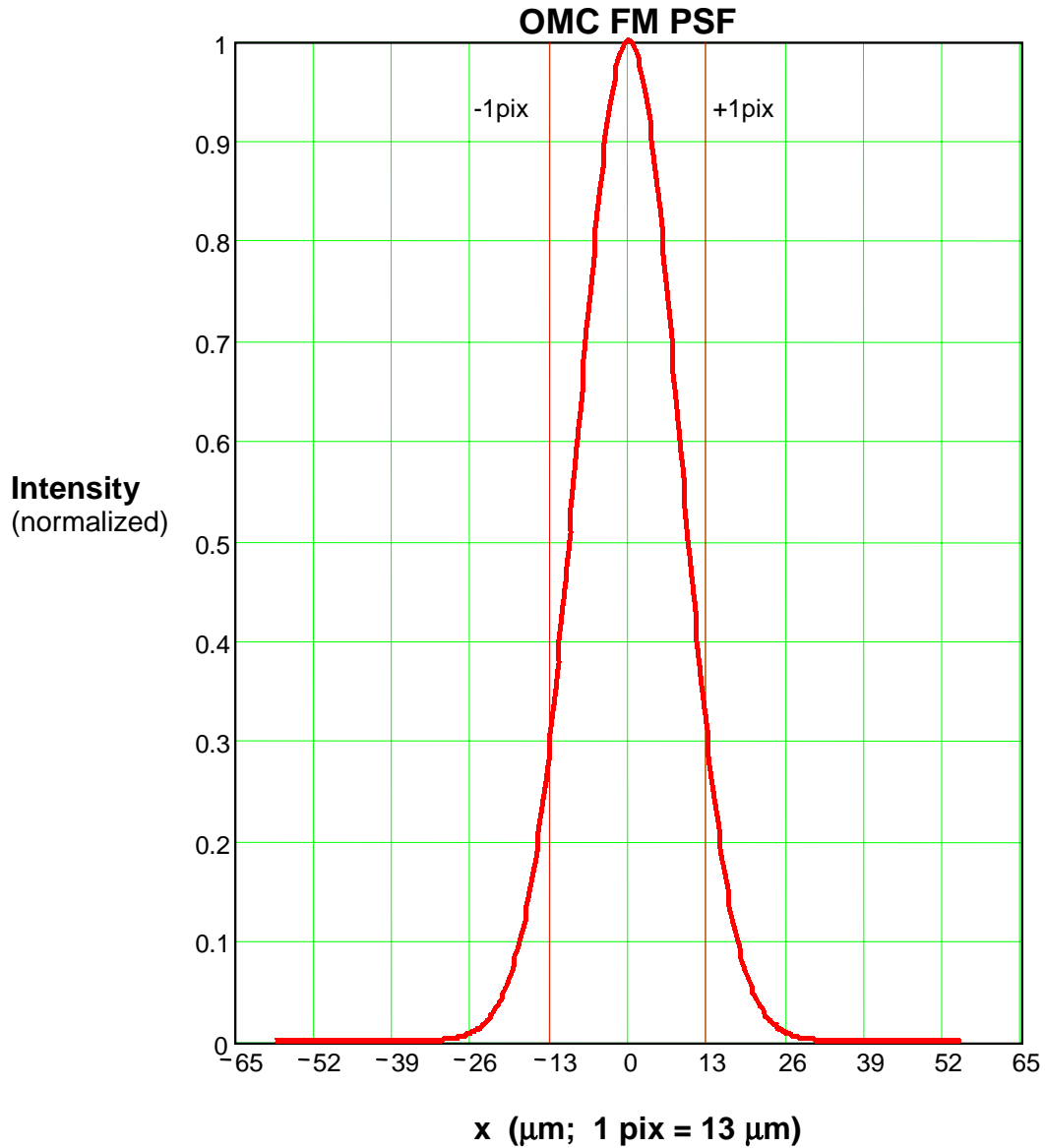
Figure 8. Point Spread Function of the OMC (optical system + detector). The plot shows a fit to the average PSF measured under different conditions. The PSF measured in orbit follows a Gaussian with FWHM \approx 1.3 pixels. More than 90% of the energy falls within a region of 3 \times 3 pixels
