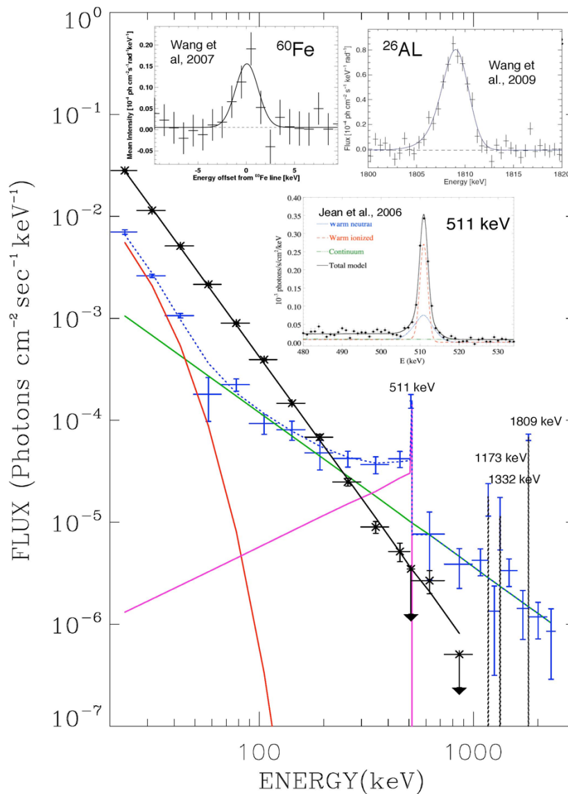
Figure 18 – SPI spectra of the galactic central radian. Black: total emission of resolved point sources; Blue: total diffuse emission; Magenta: 511 keV annihilation radiation (positronium continuum and line emission); Green: emission from the galactic ridge resulting from interstellar particle interaction; Red: accreting magnetic white dwarfs. The vertical dotted lines indicate the positions of narrow lines. Inserts show the fine spectroscopy analysis of selected lines (Jean et al. 2006, A&A 445, 579; Wang et al. 2007, A&A 469, 1005; Wang et al. 2009, A&A 496, 711; from the SPI team).
