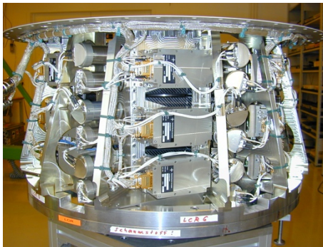
Figure 2 - View of some subsystems of the spectrometer: a) coded mask; b) detector plane; c) lower collimator ring, side view; d) rear shield assembly.
