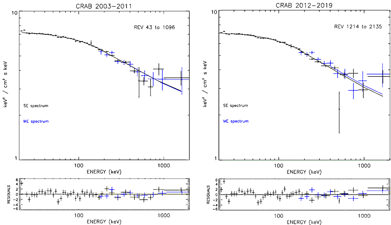
Figure 13 - SPI spectrum of the Crab (single and double events) in two different periods, obtained during the Crab calibration observations carried out between 2003 and 2019, showing the stability of the calibration of the instrument. The spectra are fit with a Band model (2 power-laws joined by a smooth curvature). The best-fit parameters of the averaged spectrum are compatible with a low-energy slope \alpha_1=1.99\pm0.01 , a high-energy slope \alpha_2=2.32\pm0.02 , a characteristic energy E_c=531\pm50 keV to describe the curvature joining both power law, and a 30-100 keV flux of 1.30 \times 10^{-8} erg/cm 2 s.
