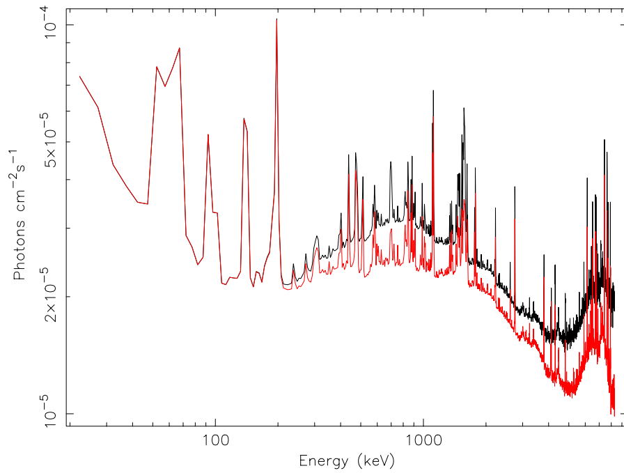
Figure 7 The narrow line (w.r.t. the instrument resolution) sensitivity of the SPI instrument for a 3 sigma detection in 10^6 seconds. Note that the 511 keV line is not shown in this figure. The lower curve (red) has multiple events included.
