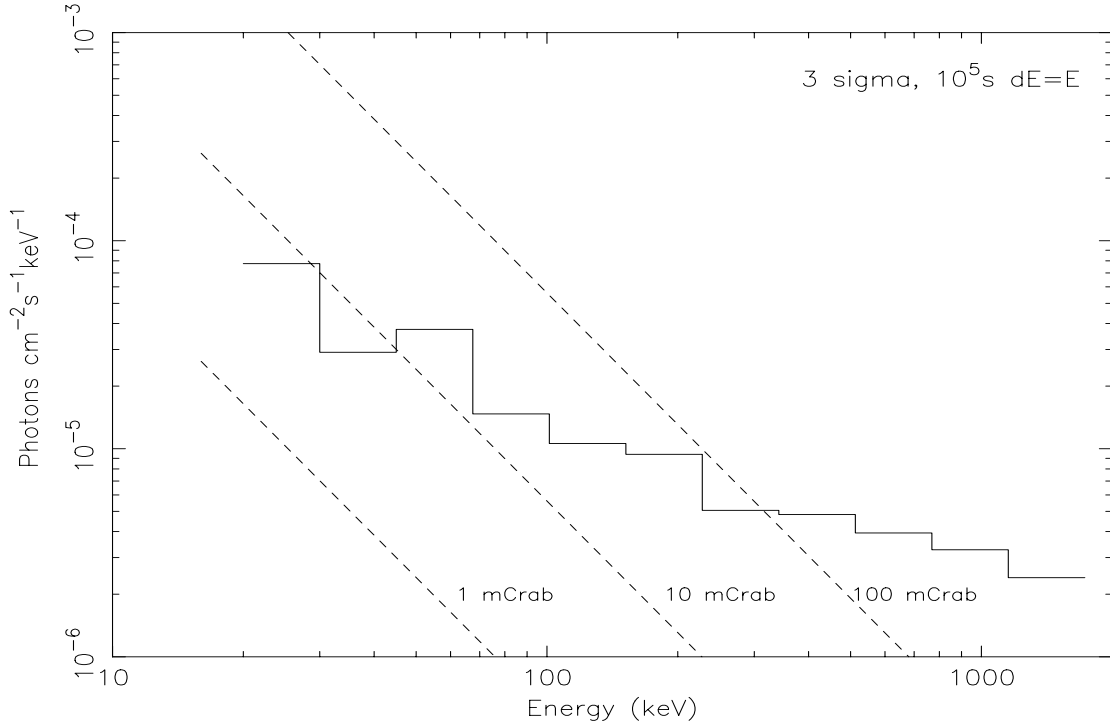
Figure 6 The continuum sensitivity of the SPI instrument for a 3 sigma detection in 10^5 seconds on-axis. The fluxes are for E/\Delta E=1 . The dashed lines indicate extrapolations from X-rays using an powerlaw with photon index -2.1 for 1, 10 and 100 mCrab.
