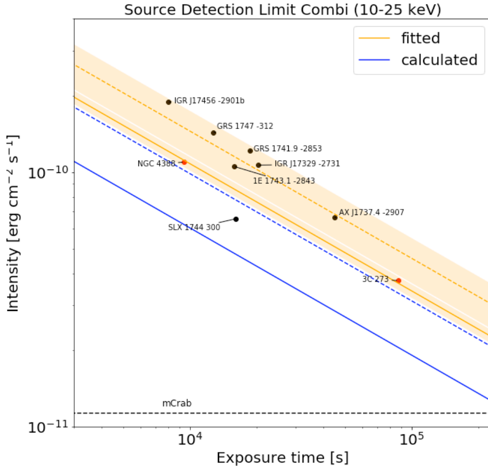
Figure 11: Same as Figure 10, but for the energy range from 10 to 25 keV.
