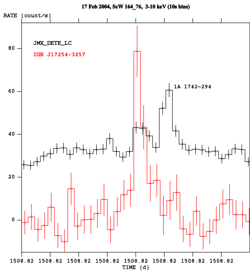
Figure 17: JEM-X detector light curve (black) and IGR J17254-3257 source light curve (red) during a 6 minute interval around the burst that occurred at UTC 19:44:00 on 17 February 2004. Note that another, stronger, burst from 1A 1742-294 occurred less than one minute after the event from IGR J17254-3257.
