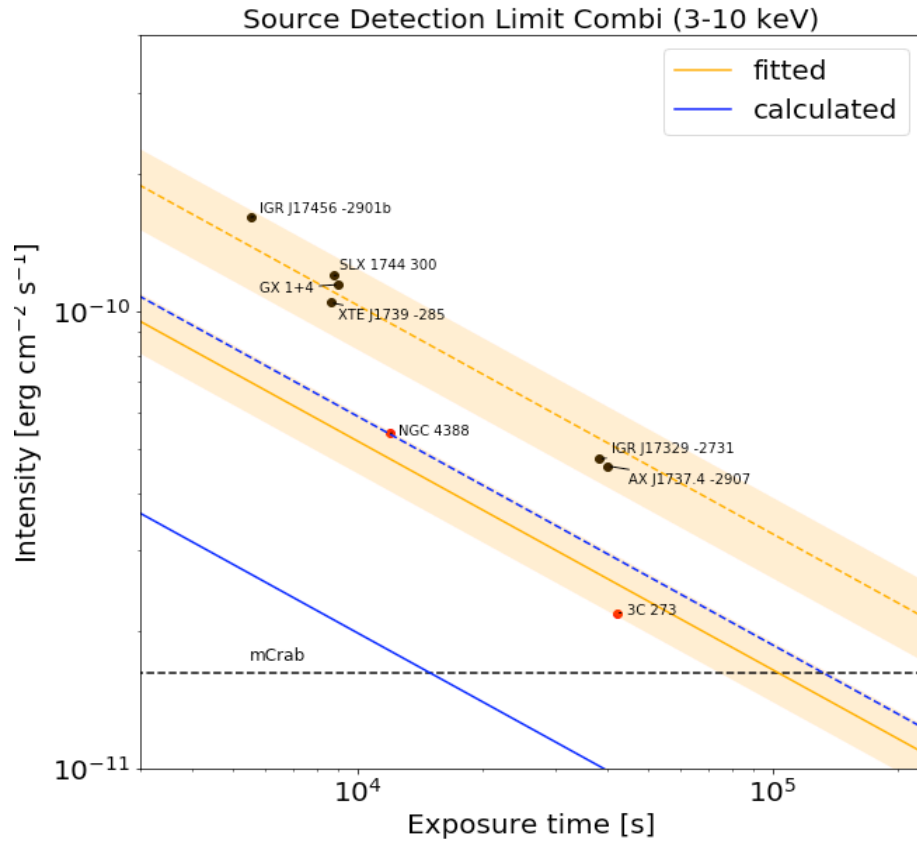
Figure 10: Source detection capabilities in the 3-10 keV energy band as a function of the effective accumulated exposure time in JEM-X mosaic images corrected for dead time, grey filter and vignetting effects. The slope of the lines is obtained from simulations where an isolated source must be detected at 3\sigma in the deconvolved image. The dashed line represents the case where there are additional sources in the field of view giving a background corresponding to a total of 1 Crab. The positions of the lines are determined by actual measurements. Examples of such actual observations are given: the source 3C 273 and the other empty circles are instances of isolated sources, while the crossed circles represent sources observed in the crowded Galactic Centre region. The \sigma values given in parentheses are obtained from a measure of the highest source pixel in significance mosaic maps with the default pixel size (1.5').
