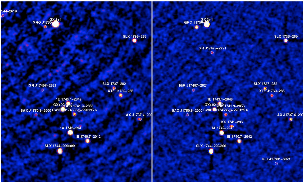
Figure 9: Deep mosaic significance image of the region around the Galactic bulge, based on over 3000 JEM-X exposures (science windows) in the 3-10 keV (left) and 10-25 keV (right)
