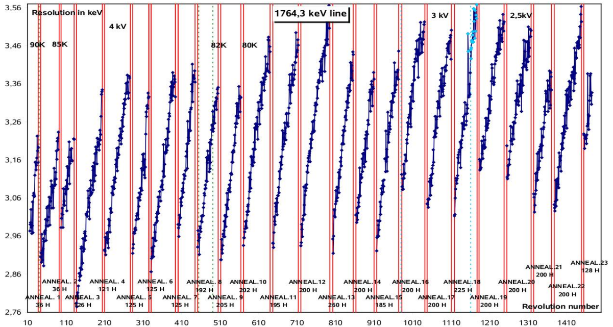
Figure 8 - The evolution of energy resolution at 1764.3 keV as a function of time in between the annealing periods (from the SPI team).
