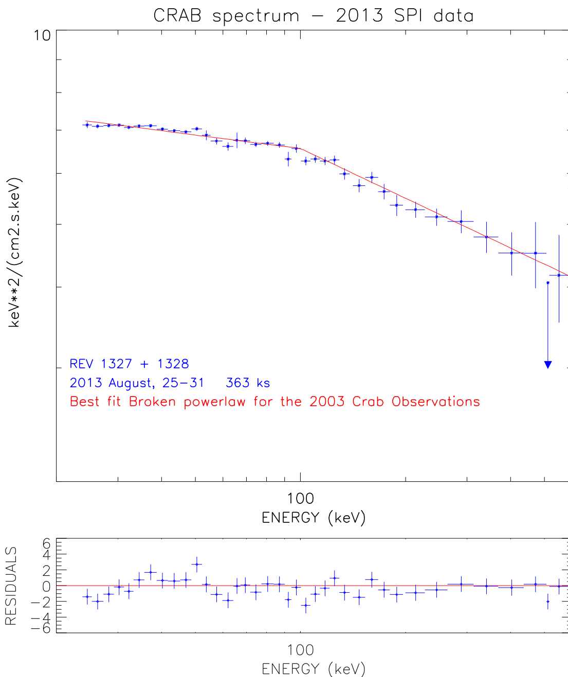
Figure 13 - SPI spectrum of the Crab obtained during the Crab calibration observations carried out in August 2013 (revs. 1327+1328) superimposed with the best fit obtained from 2003 observations (revs. 43+44+45) demonstrating the stability of the SPI instrument. The best fit model is a broken power-law (break energy fixed to 100 keV) with indexes of 2.07 and 2.26 and 100 keV flux of 6.6 \times 10^{-4} photons \text{cm}^{-2} \text{keV}^{-1} .
