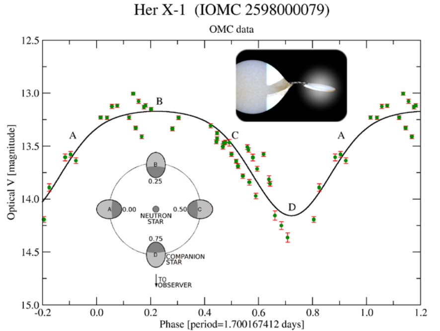
Figure 17: OMC light curve of the low-mass X-ray binary Her X-1 (see Figure 16) folded on the 1.7 days orbital period (Risquez et al. 2008, PoS(Integral08)129).
