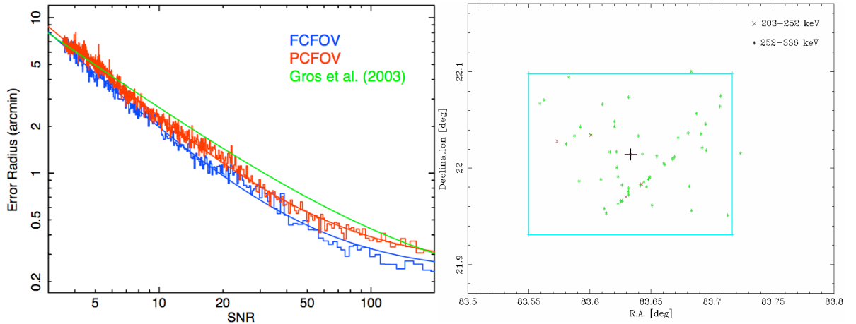
Figure 10: Left panel: ISGRI point source location accuracy (PSLA; 90% confidence level) in units of arcminutes for sources in the FCFOV using an analysis based on ~40000 science windows is given by: 31.1(\text{SNR})^{-1.25} + 0.23 (Scaringi et al. 2010, A&A, 516, 75). The resulting fits are shown for the FCFOV (blue) and the PCFOV (red), and are compared with the only previous determination of the PSLA by Gros et al. (2003, A&A, 141, L179), that parametrized their fit as: 22.1(\text{SNR})^{-0.95} + 0.16 . Right panel: PICsIT PSLA using Crab observations from revolutions 39, 43, 44 and 45. Results for 2 energy bands are given (203–252 keV and 252–336 keV). Only detections with at least 3\sigma in a science window (or exposure) are used. The catalog position of the Crab is marked by a cross, and the size of a PICsIT pixel (10') is indicated by the rectangle.
