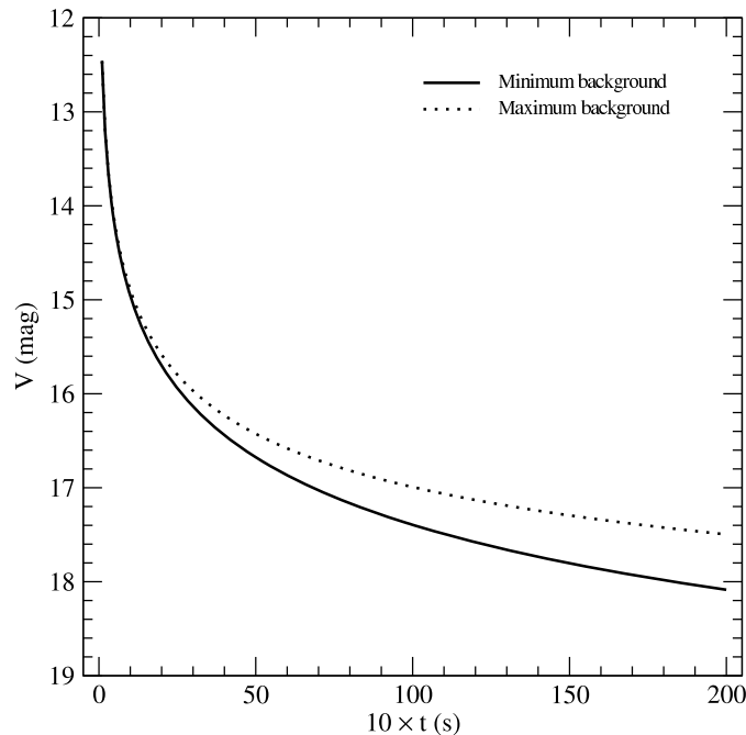
Figure 9: Limiting faint magnitude for a 3\sigma detection in the V band as a function of integration time. The best and the worst background cases are shown. It is assumed that 10 separate
