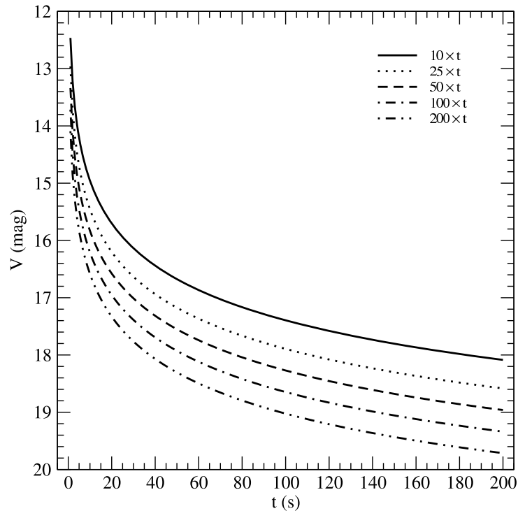
Figure 10: Limiting faint magnitude for a 3\sigma detection in the V band as a function of integration time. Best case background conditions are assumed (galactic pole, no zodiacal light). The curves correspond to different total numbers of images being combined.
