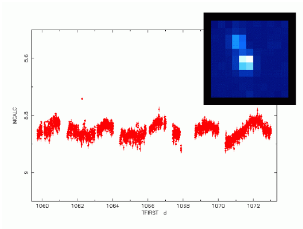
Figure 14: OMC light curve of high-mass X-ray binary Cygnus X-1 obtained using single exposures of 10 and 30 s. The OMC sub-window for this source is shown on the upper right corner of the graph. Time is in INTEGRAL Julian days. (Credits: OMC Team)
