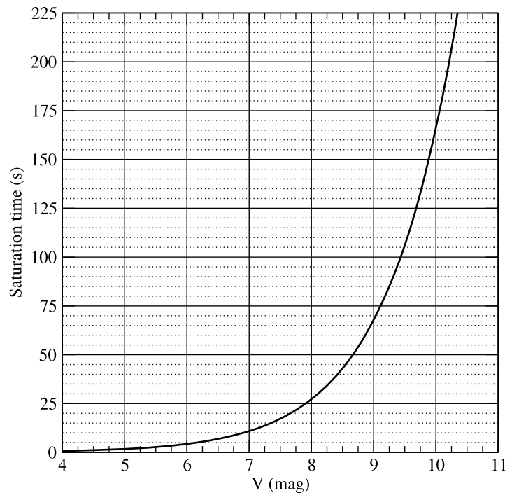
Figure 12: CCD saturation time as a function of V magnitude. Note that for integrations of 50 s, all stars with m_V < 8.6 will saturate the CCD. For the shortest OMC integration times (fast monitoring mode: 3 s), the brightest stars that can be observed should be fainter than m_V > 5 .
