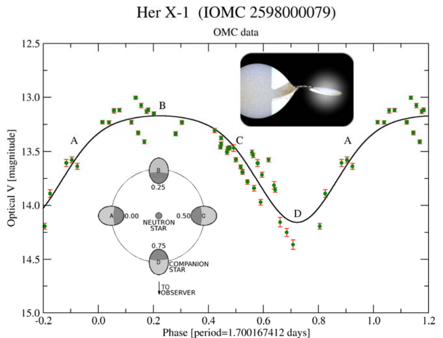
Figure 17: OMC light curve of the low-mass X-ray binary Her X-1 (see Figure 16) folded on the 1.7 days orbital period (Risquez et al. 2008, PoS(Integral08)129).
