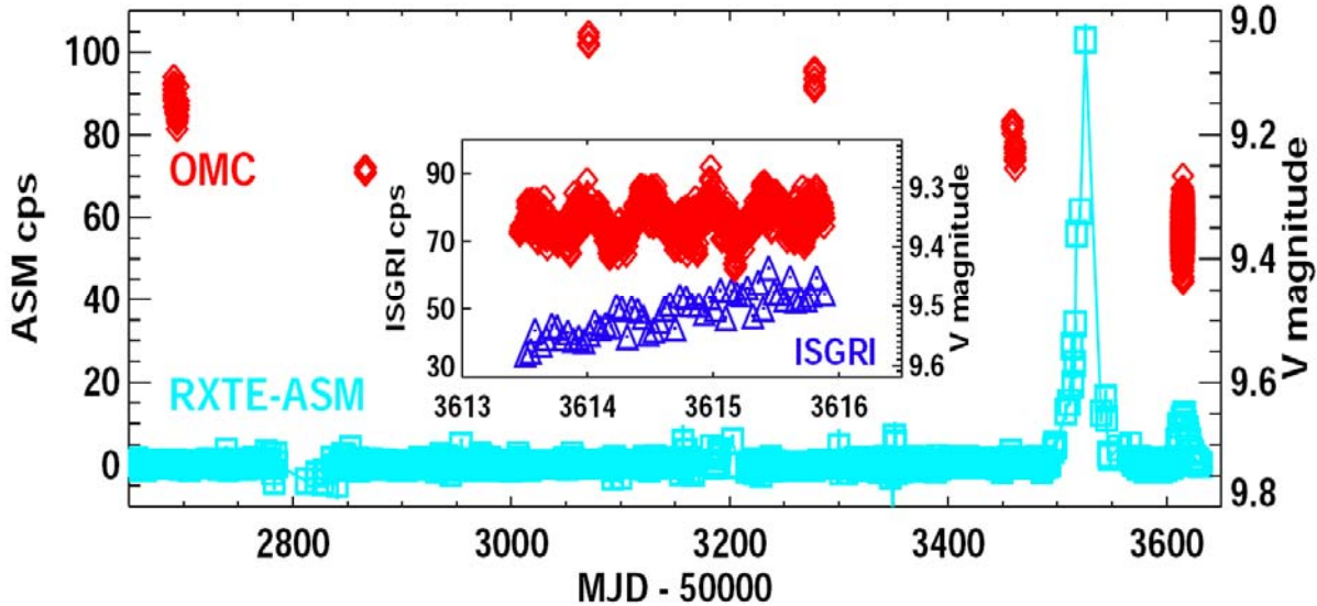
Figure 18: Long-term light curves of the Be/X-ray binary and accreting pulsar 3A0535+262/HD 245770 obtained with the RXTE/ASM (left Y-axis) and the INTEGRAL/OMC (right Y-axis). The inset shows the OMC and ISGRI light curves during the INTEGRAL Target of Opportunity observations around MJD 53613-53616. (Taken from Kretschmar et al. 2006, ESA SP-604, p. 273)
